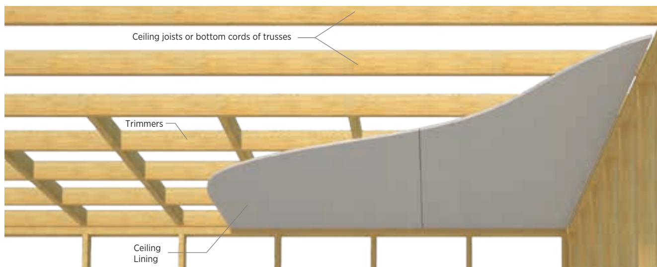
Figure 15: Direct Fixed Ceiling
