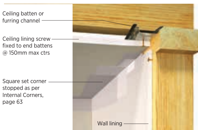
Figure 45: Square Set
