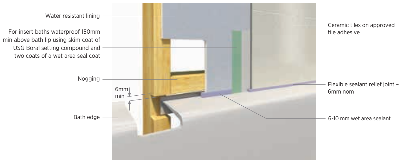
Figure 62: Bath and wall junction
