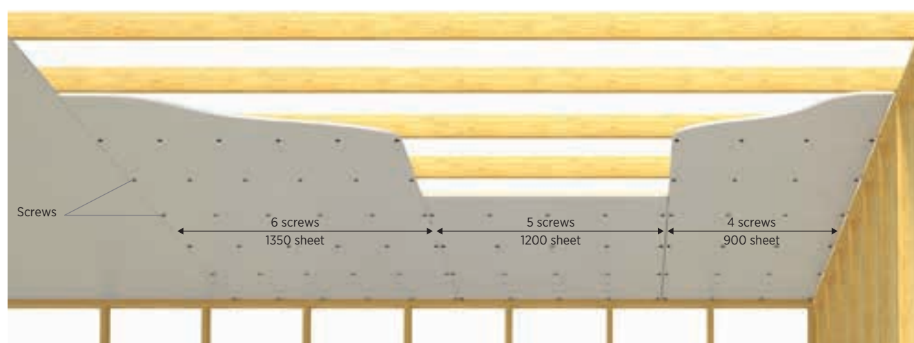
Figure 21: Screw fixing (only) layout for ceilings
