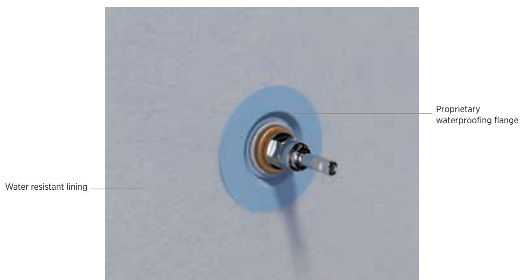
Figure 68: Plumbing Penetrations With Proprietary Waterproofing Components
