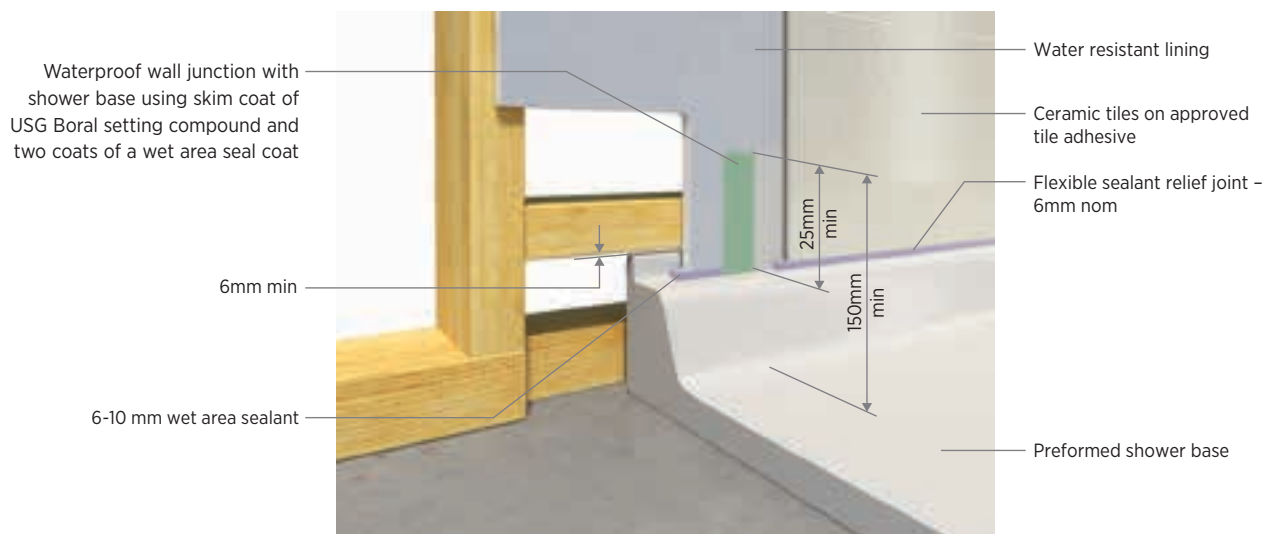
Figure 63: Preformed shower base and wall junction
