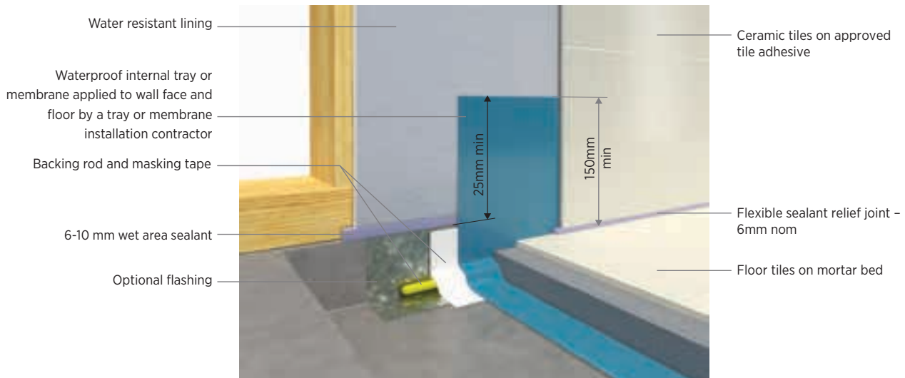
Figure 65: Set-down shower base and wall junction
