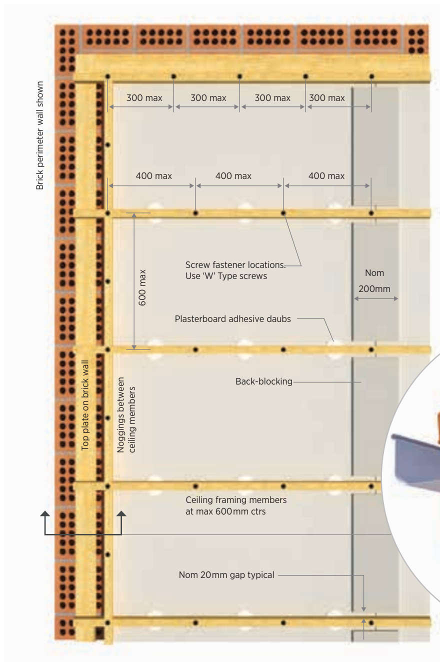
Figure 26: Garage ceiling fixing layout (1200mm wide plasterboard sheets shown)
