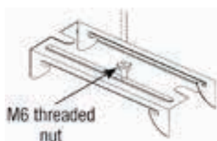
Figure 48: Masonry fixing clips
