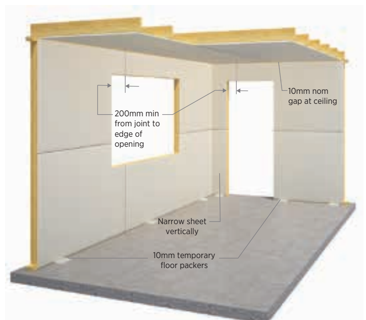
Figure 13: Room Layout Option 2
