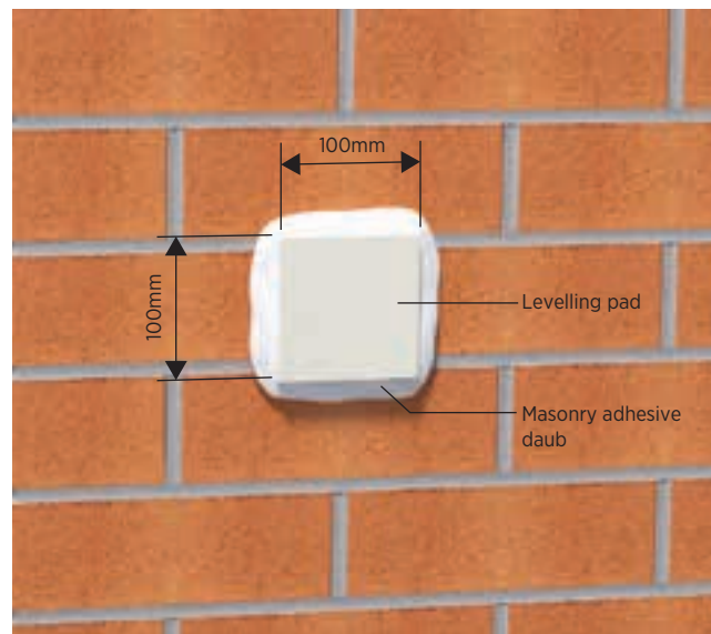
Figure 47: Levelling pads
