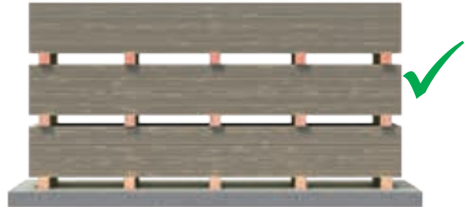
Figure 8: Correct placement of billets
