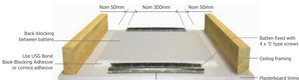
Figure 23: Back-blocking using BackBlock™ batten
