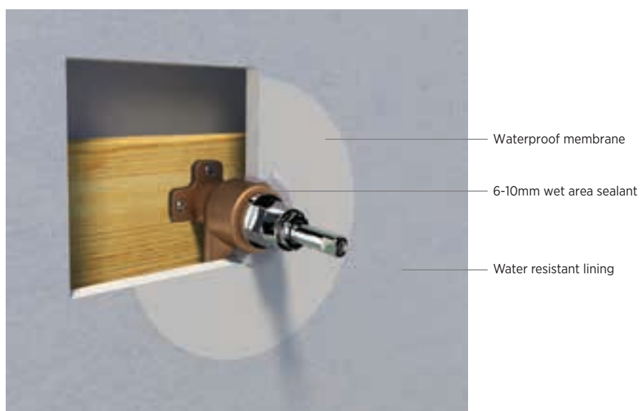
Figure 67: Plumbing Penetrations – Sealed
