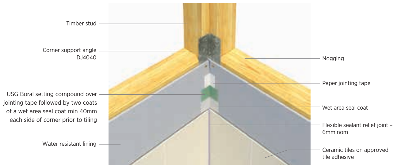
Figure 61: Internal Corner
