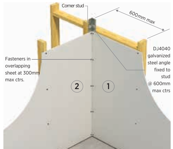
Figure 33: Internal Corner
