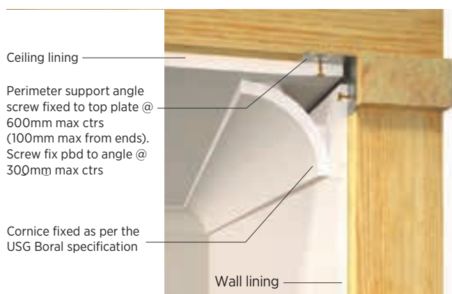
Figure 41: Cornice Detail 2 (perimeter supporting angle)
