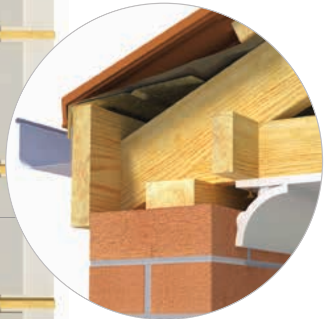
Perimeter Detail
