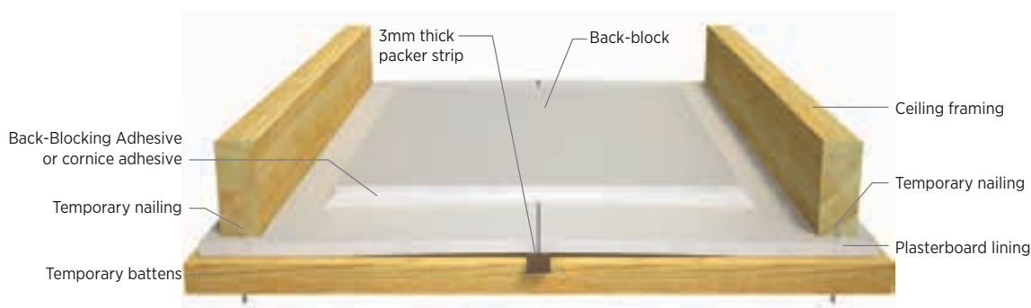
Figure 24: Back-blocking using temporary batten and packer
