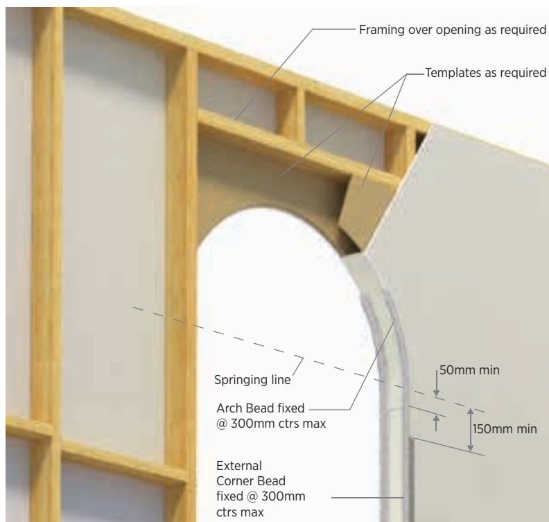
Figure 70: Arch construction
