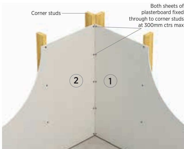
Figure 32: Internal Corner
