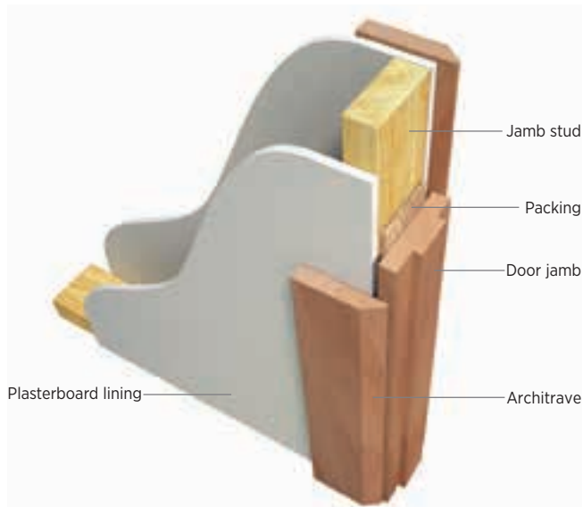
Figure 37 Door Jamb With Architraves
