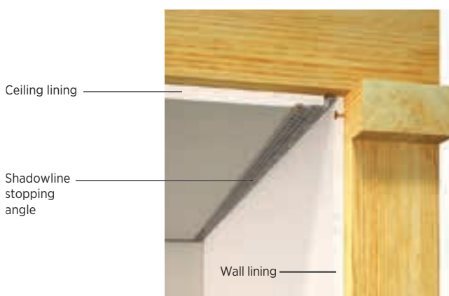
Figure 44: Shadowline Angle 2
