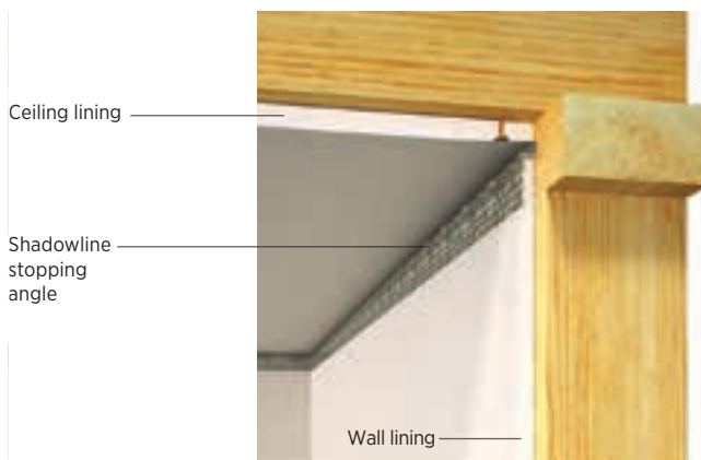
Figure 43: Shadowline Angle 1
