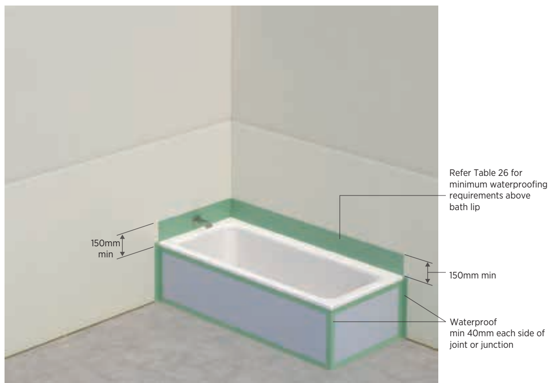
Figure 57: Waterproofing of bath
