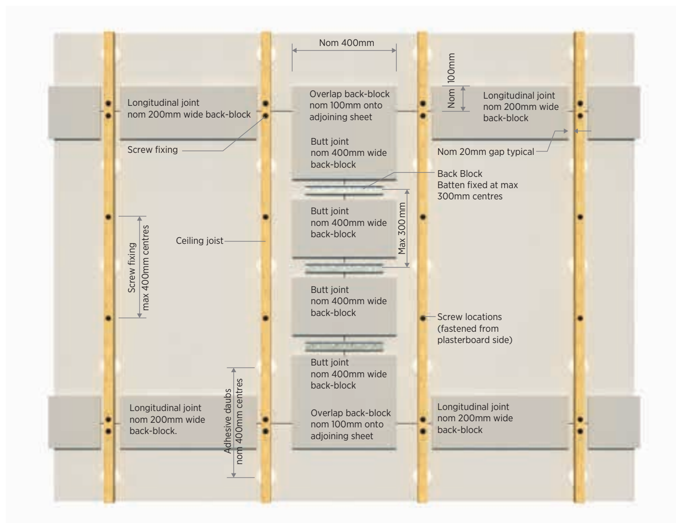
Figure 25: Back-blocking using battens — Plan view
