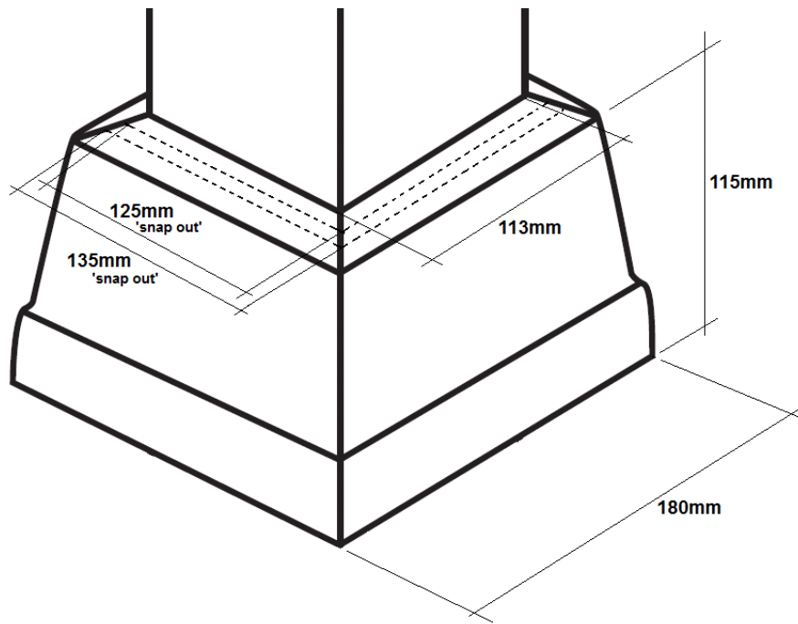
LMDKT – Large Modtrim Post Cover & Support
