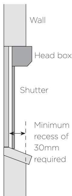
In-reveal side view with sill
