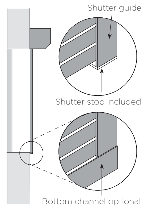
On-wall side view with no sill
