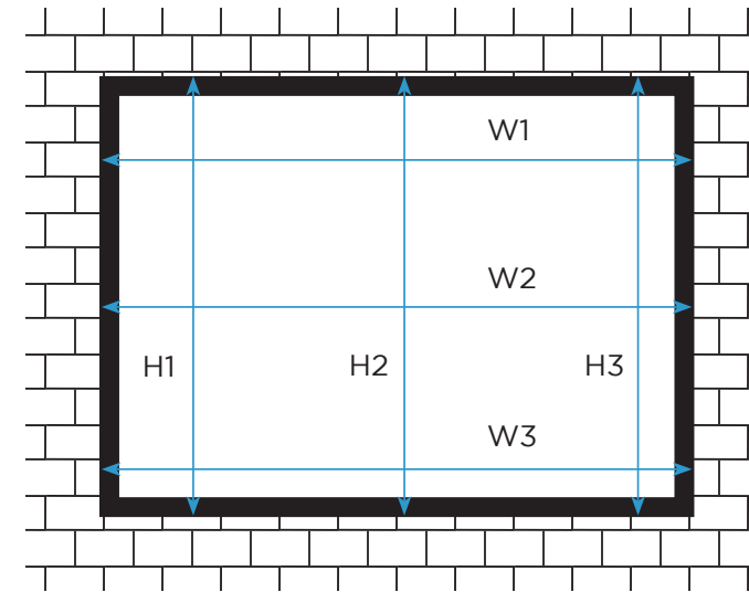
Window with architrave
