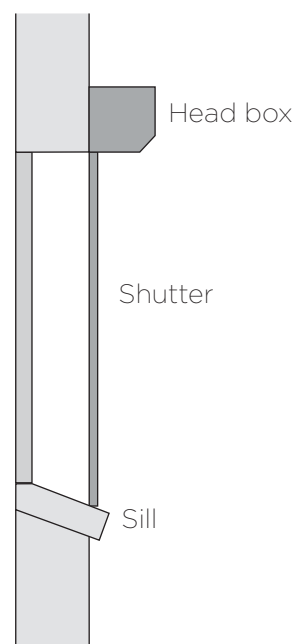
On-wall side view with sill
