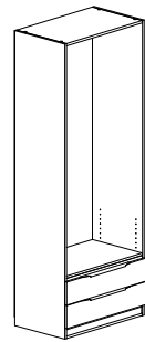
EXC-750H2 2000H x 750W x 450D 1 Hanging Rail 1 Fixed Shelf 2 Standard Drawers
