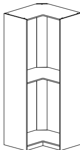
EXC-CNR-Hanging 2000H x 800W x 450D 2 Hanging Rails
