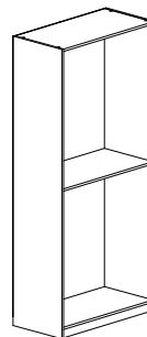
EXC-900 2000H x 900W x 450D 2 Hanging Rails
