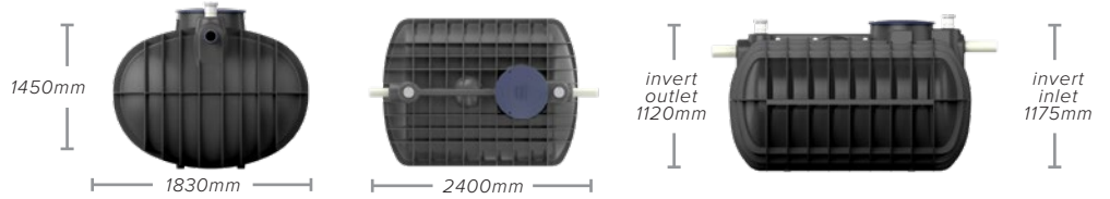
MODEL UST4500 4500L CAPACITY
