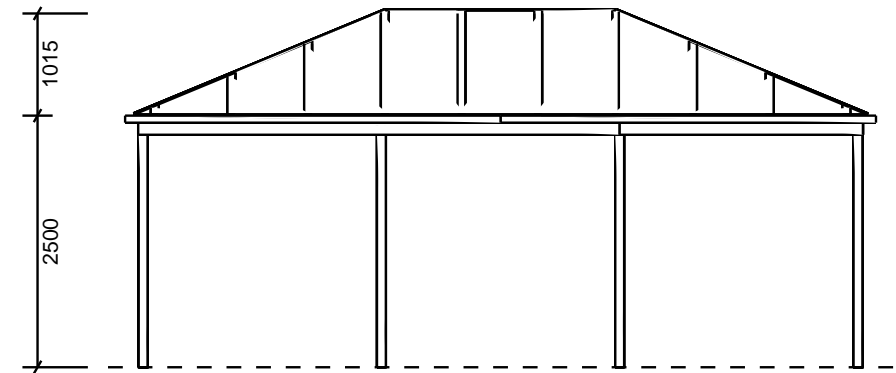
RIGHT ELEVATION 1:75
