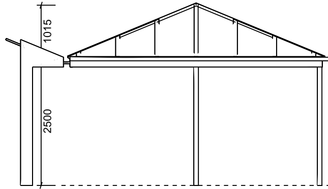
FRONT ELEVATION 1:75
