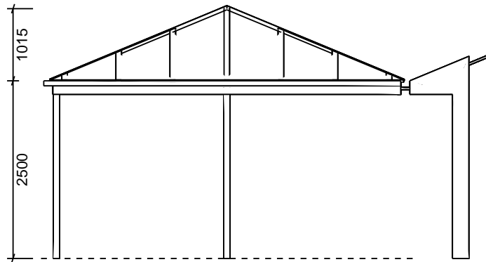
BACK ELEVATION 1:75
